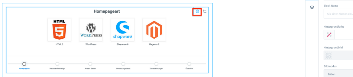
Figure 4: Open Settings
